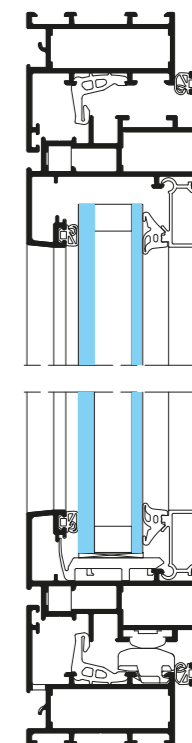
Verticale
