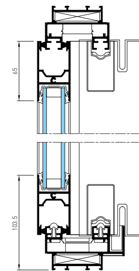
Verticale
