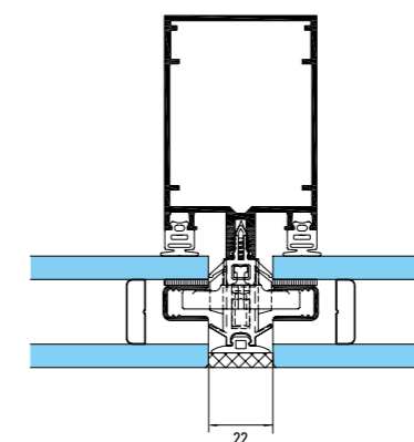
Vitrage structural
