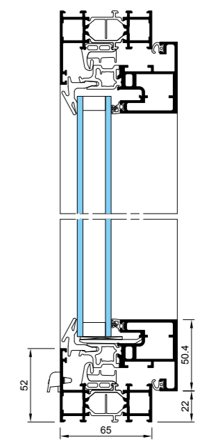
Verticale
