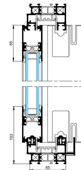
Verticale
