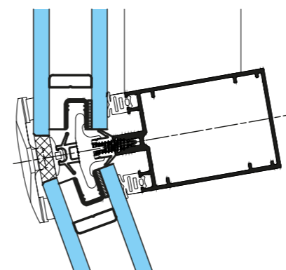
Facette +/- 10°
