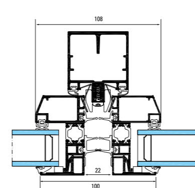
GEODE VEP parties fixes vision
