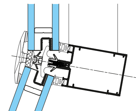
Facette +/- 10°
