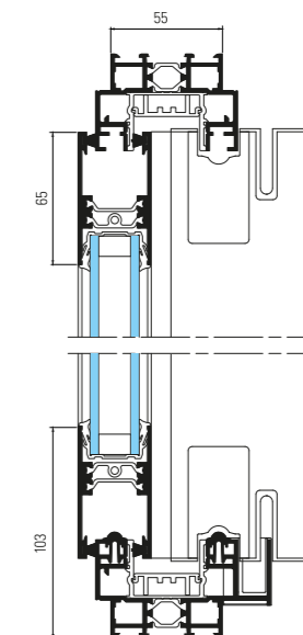
Verticale
